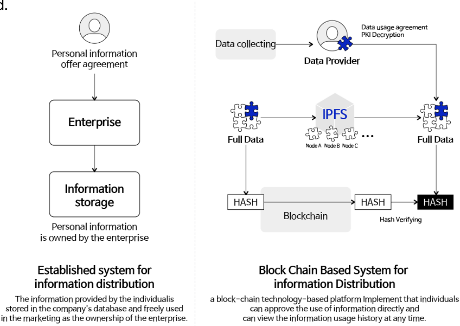
Picture 23. Block Chain Based System for Information Distribution (Right)
