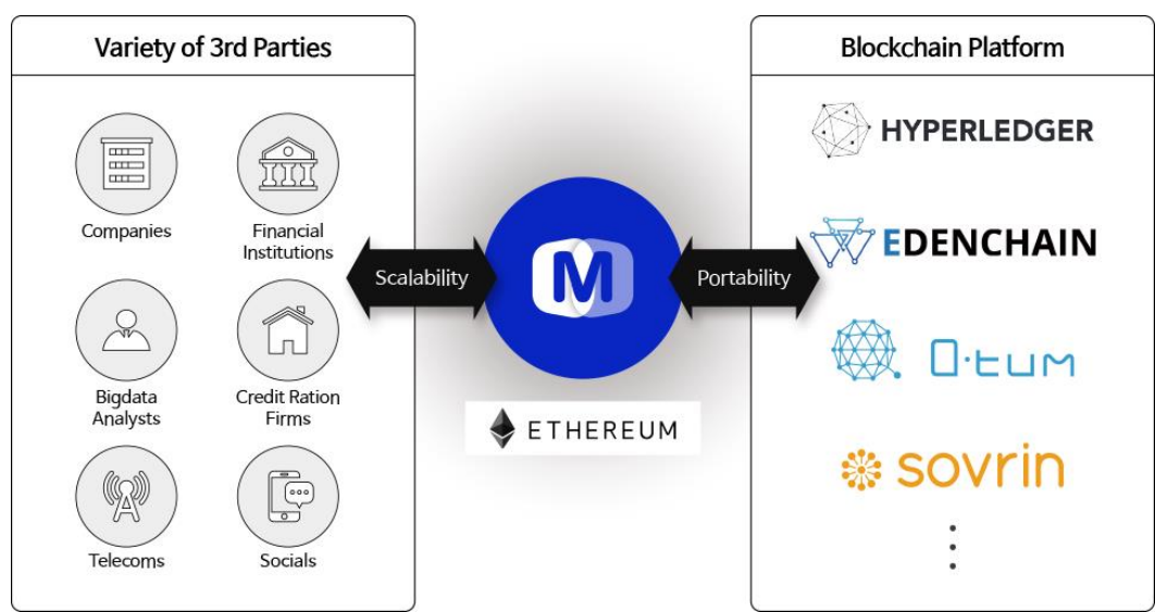
Picture 27. Scalability
